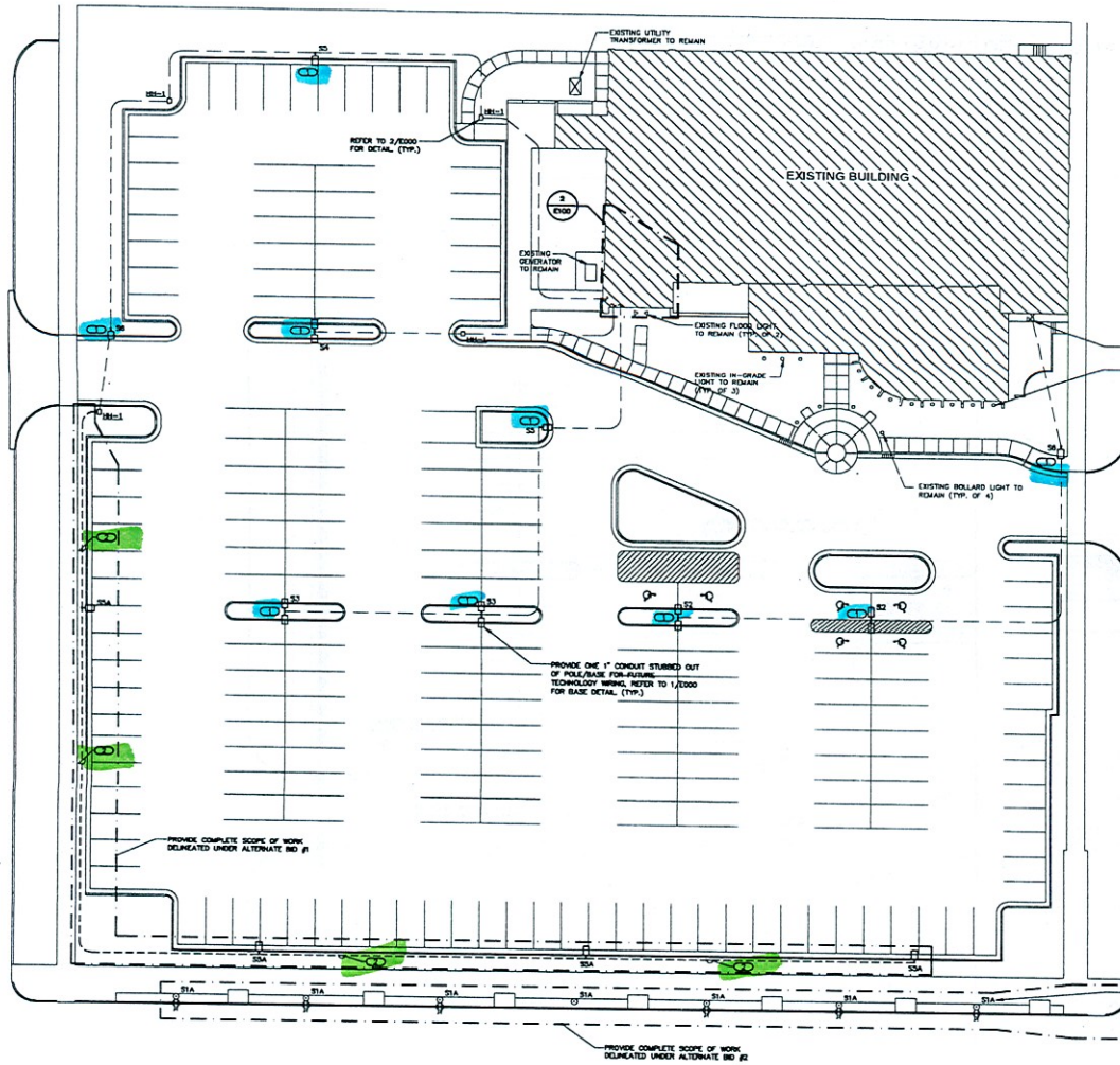
1 SITE PLAN - ELECTRICAL SCALE: 1/8"=1'-0"
